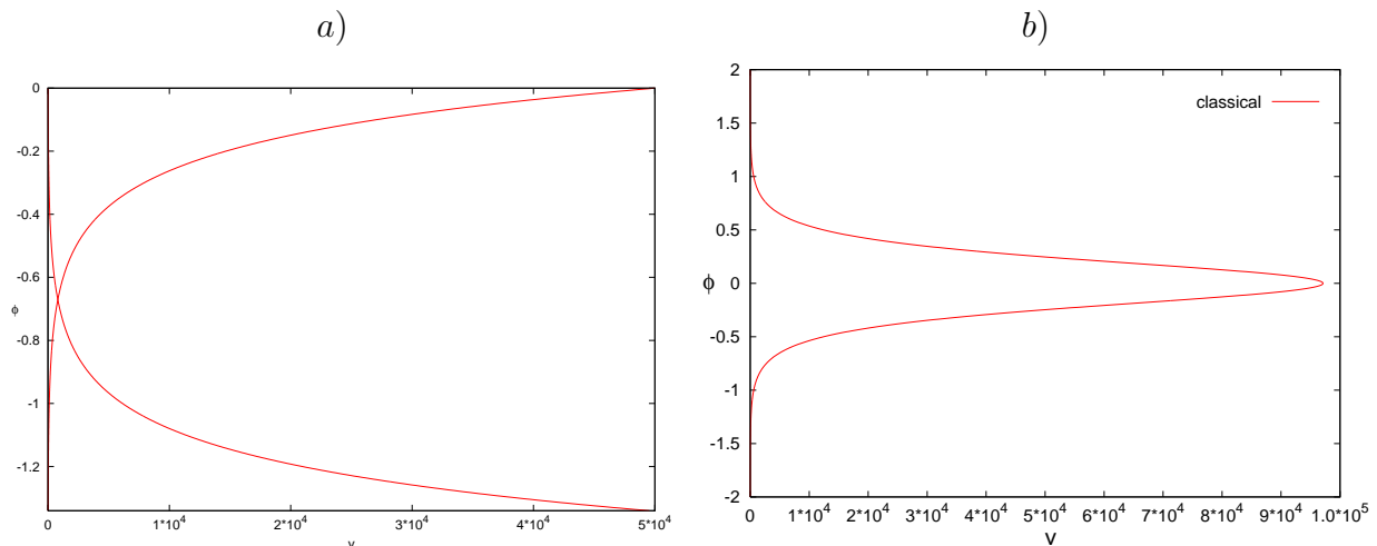
FIG. 1: Dynamics of FLRW universes with zero cosmological constant and a massless scalar field. Classical trajectories are plotted in the v - \phi plane, where v denotes the volume and \phi the scalar field. a) k=0 trajectories. b) A k=1 trajectory.
